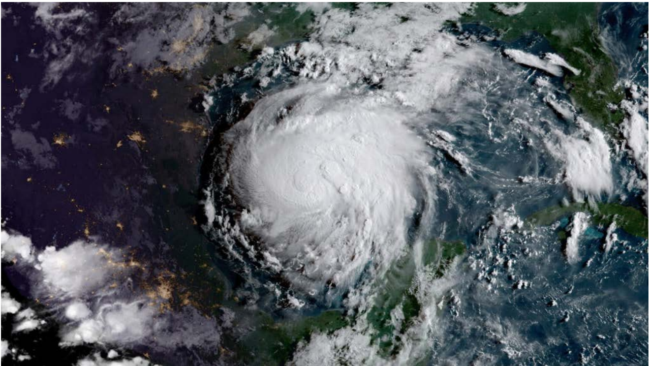
Hurrikaani Harvey.
